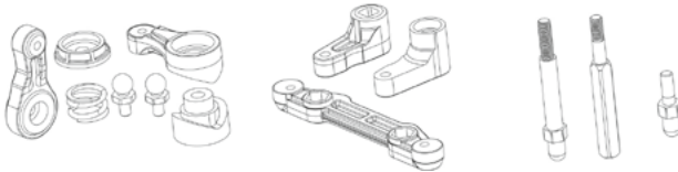
500405932 Servo Saver- Lenkhebel-Set, Expl. 013 Servohebel / Servo Saver set, steering plate, post
